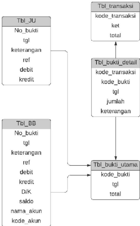
Gambar 2: Entity Relationship Diagram
