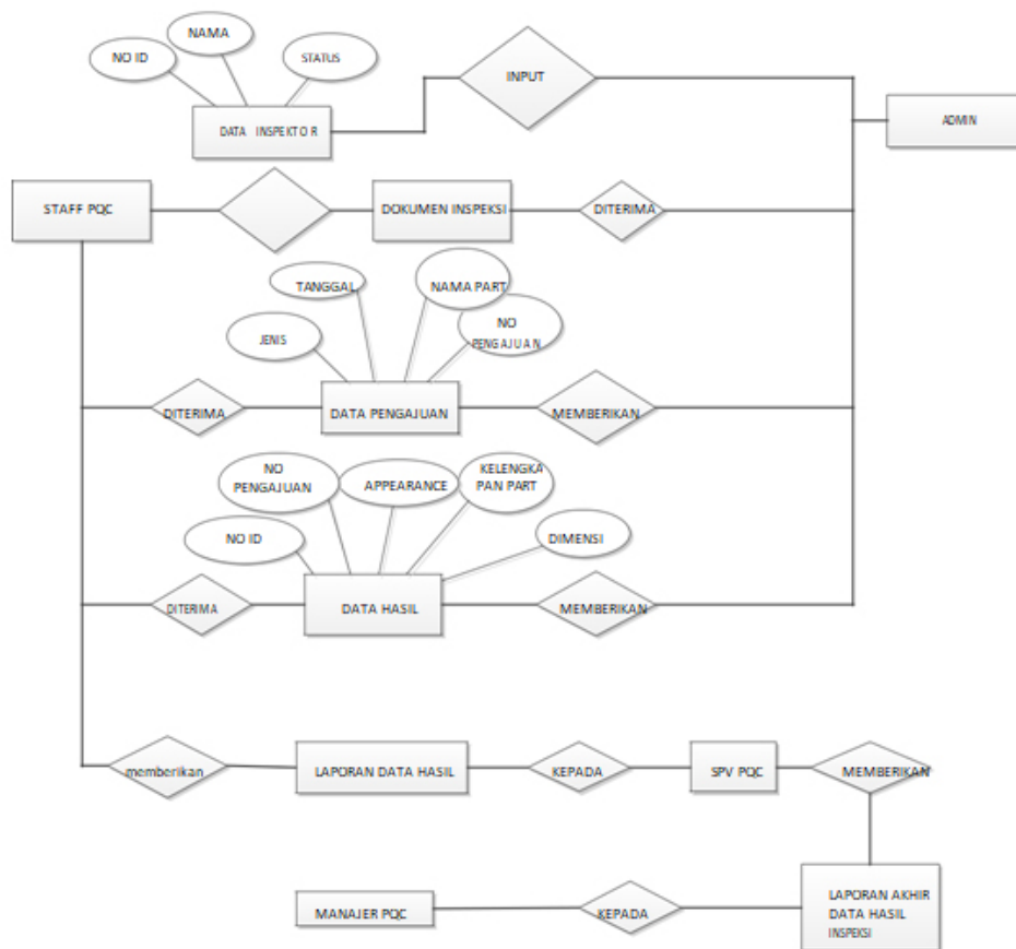
Gambar 5: Entity Relasionalship Diagram Sistem Inspeksi
