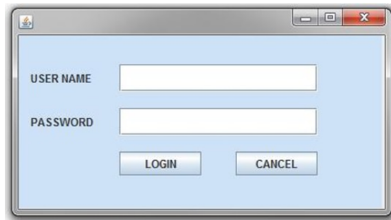
Gambar 6: Tampilan Login
